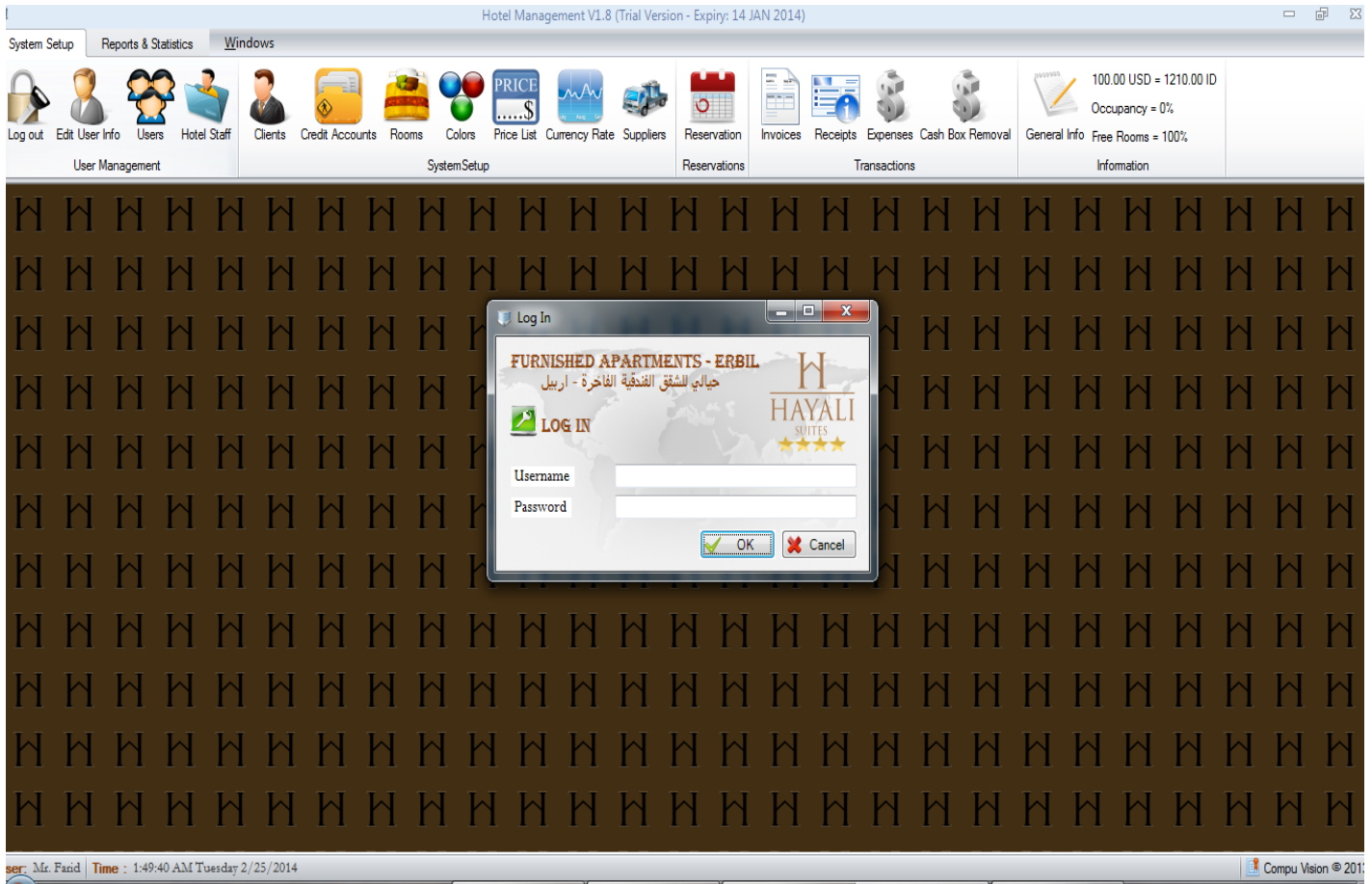
Fig. 1: Main Page
